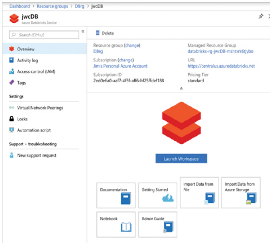
FIGURE 3-17 An instance of Azure Databricks in the Azure portal
