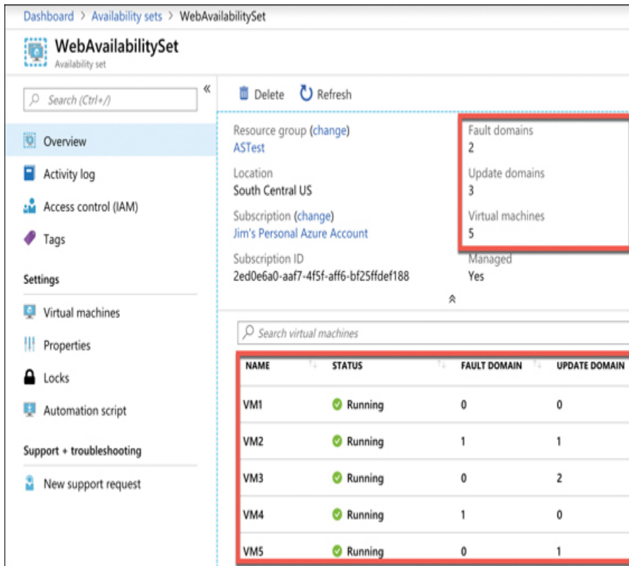
FIGURE 2-19 An availability set in the Azure portal showing fault domains and update domains
