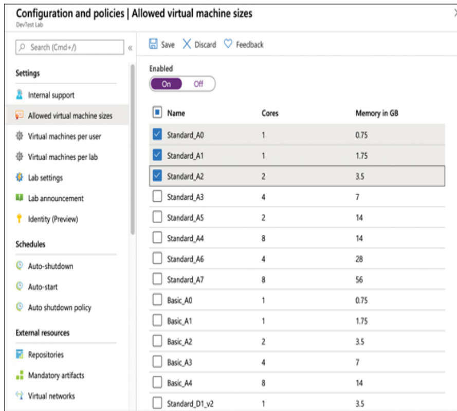
FIGURE 3-58 Configuring a policy for allowed virtual machine sizes
