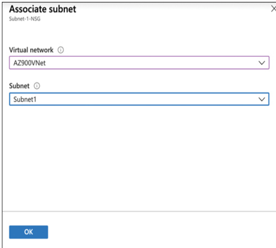
FIGURE 4-26 Associating an NSG with a subnet
