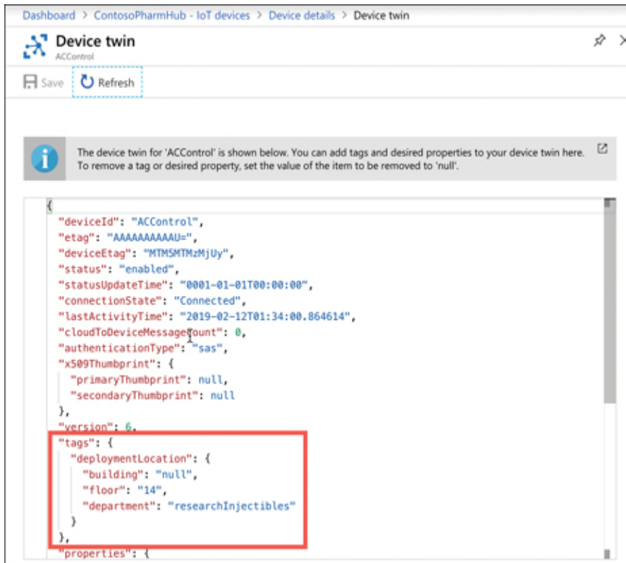
FIGURE 3-2 Device twin showing tags set in the JSON
