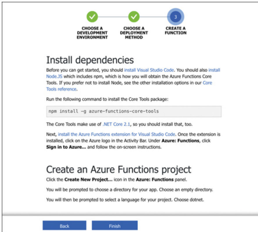
FIGURE 3-37 Creating a function using Visual Studio Code and Azure Functions Core Tools
