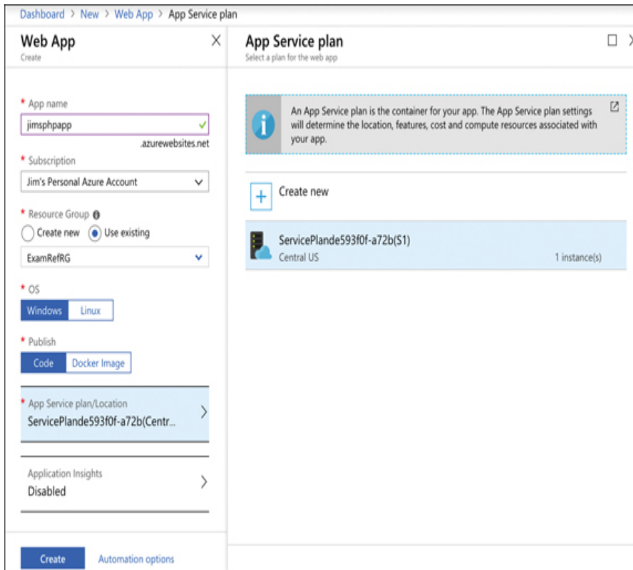
FIGURE 1-4 Creating a web app in Azure App Service
