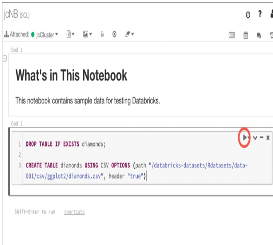
FIGURE 3-22 Adding code and running a command
