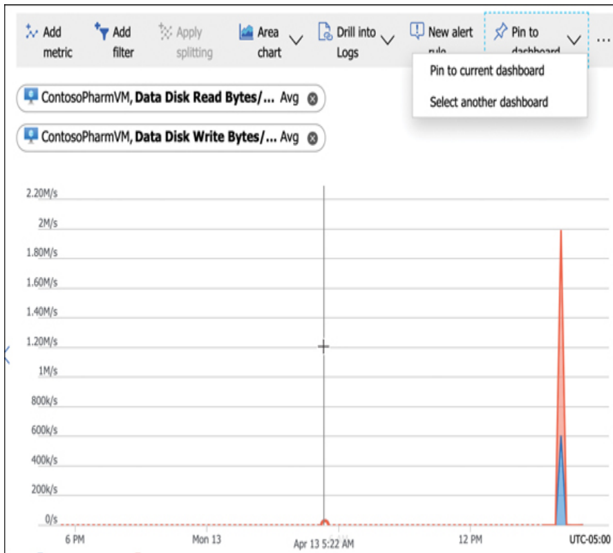
FIGURE 3-92 Pinning a chart
