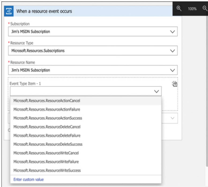
FIGURE 3-47 Events for an Azure subscription
