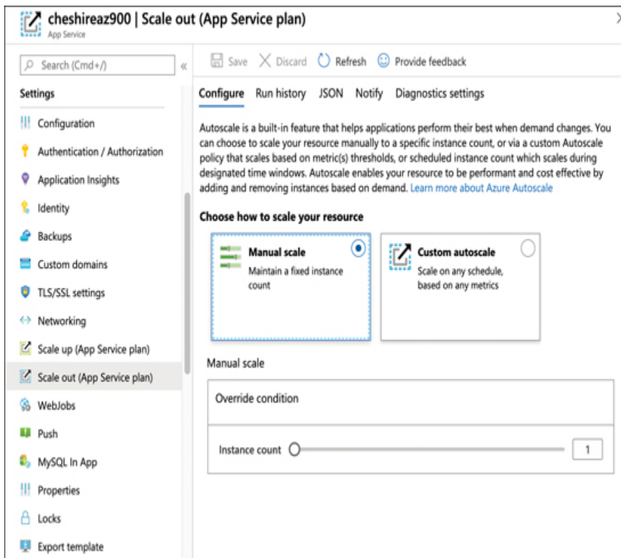
FIGURE 2-23 Settings for a web app make it easy to add features and scale your app
