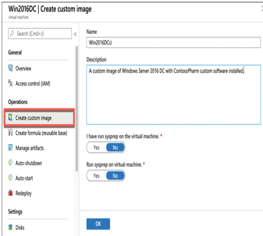
FIGURE 3-55 Creating a custom image in DevTest Labs
