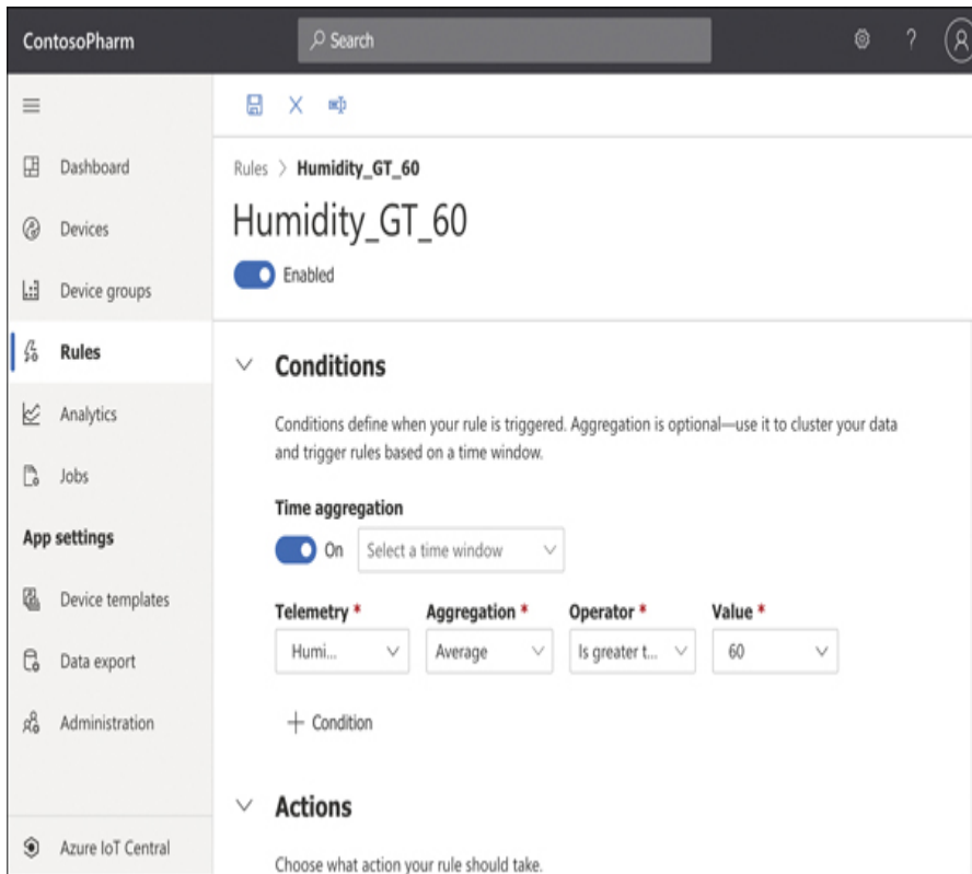
FIGURE 3-12 Creating a rule
