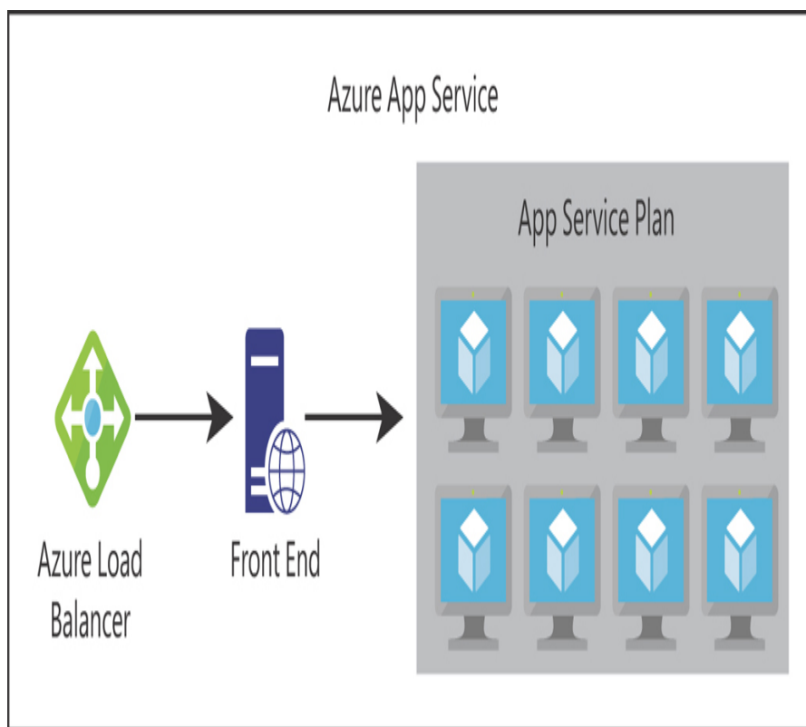
FIGURE 2-20 A high-level representation of Azure App Service
