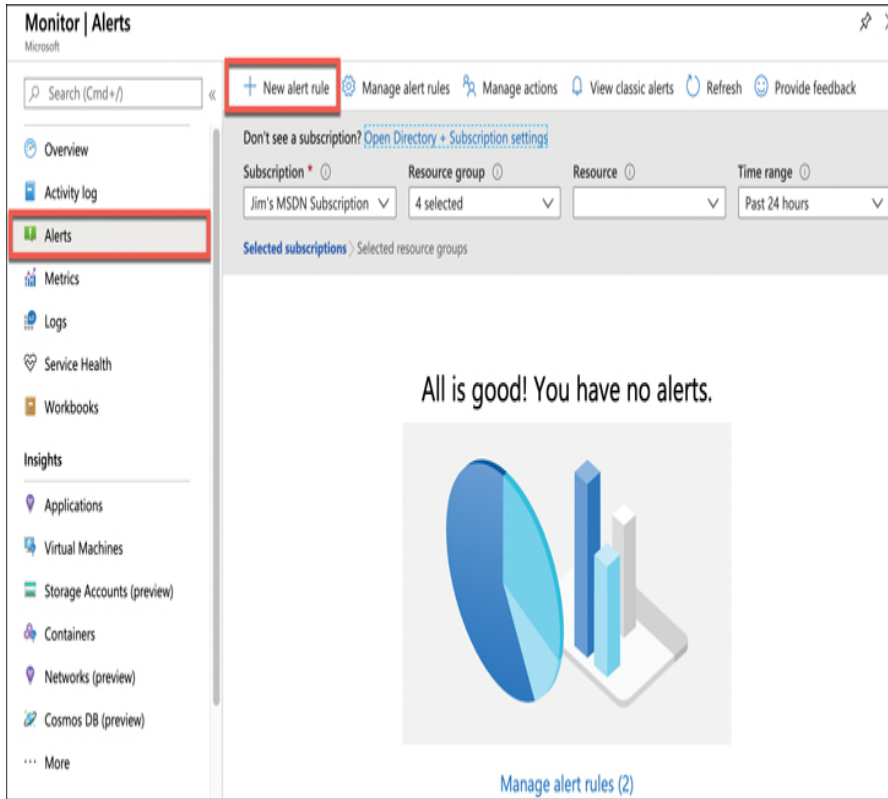
FIGURE 3-93 Creating an alert rule
