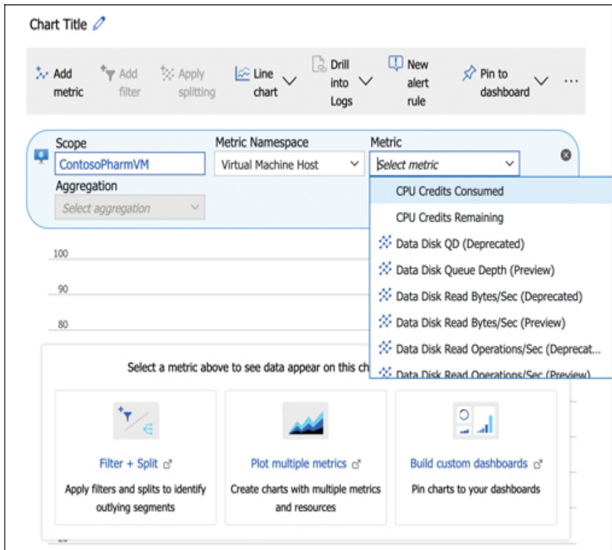
FIGURE 3-88 Metrics for VMs
