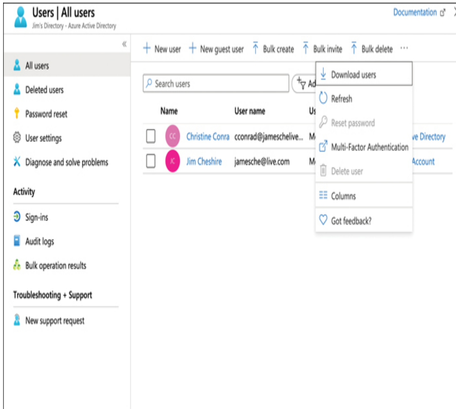
FIGURE 5-9 Enabling multifactor authentication
