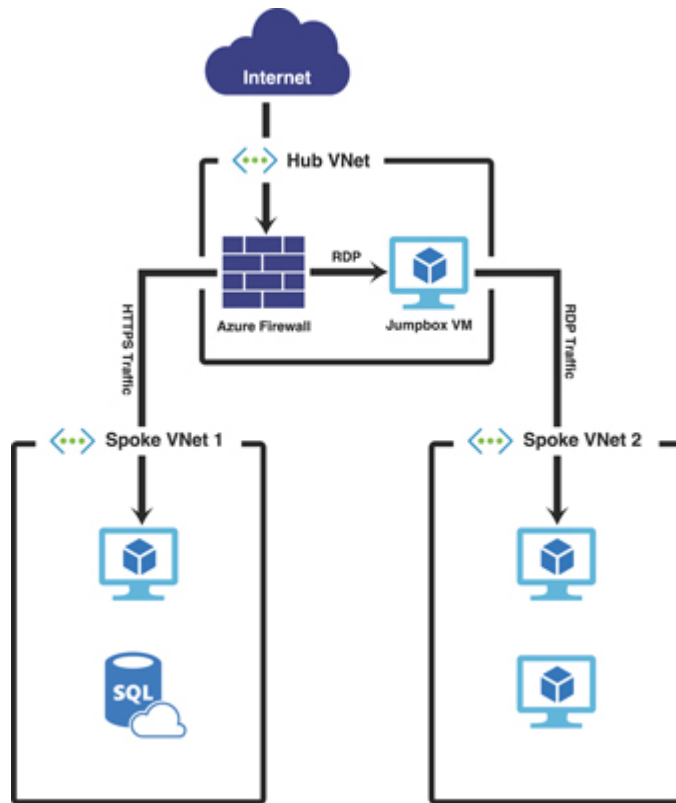
FIGURE 4-28 An example of a hub and spoke network configuration with Azure Firewall
