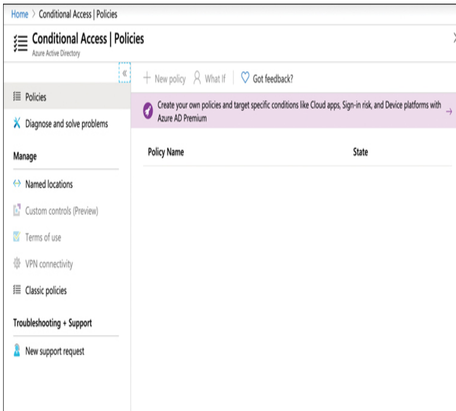
FIGURE 5-8 The Conditional Access policies blade in the Azure portal
