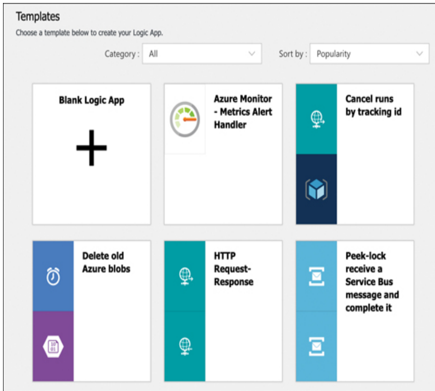
FIGURE 3-40 Logic App templates
