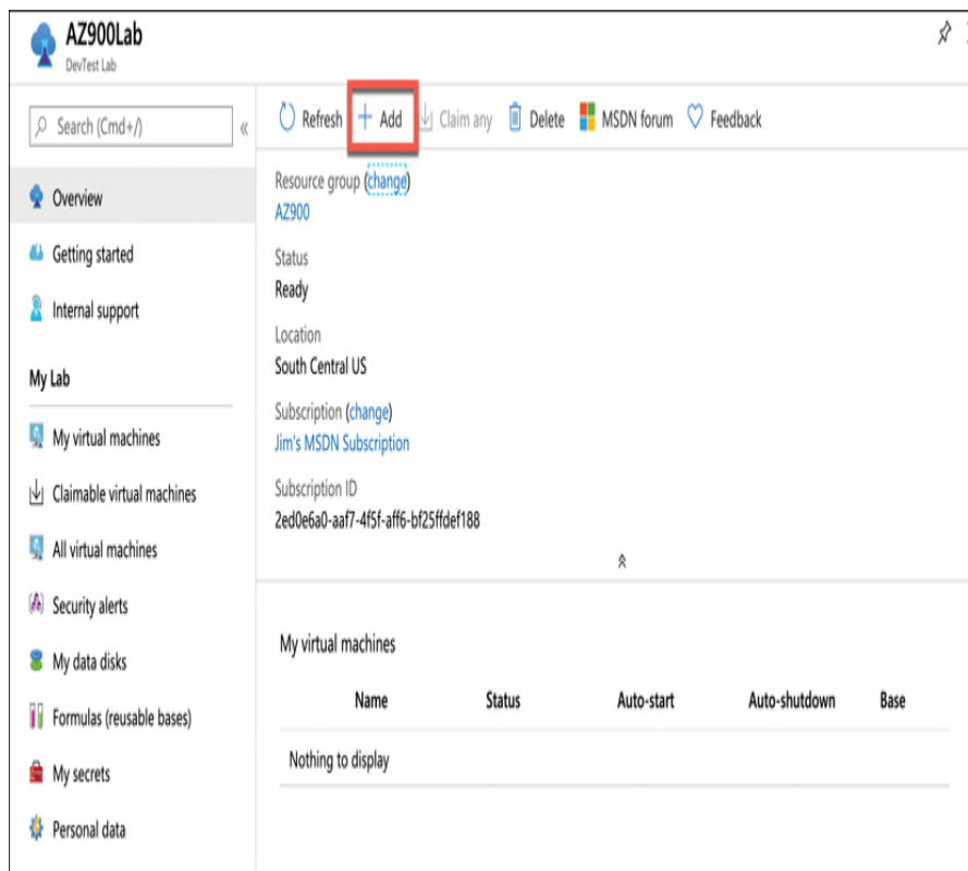
FIGURE 3-52 Click Add to add a new VM to a DevTest Lab
