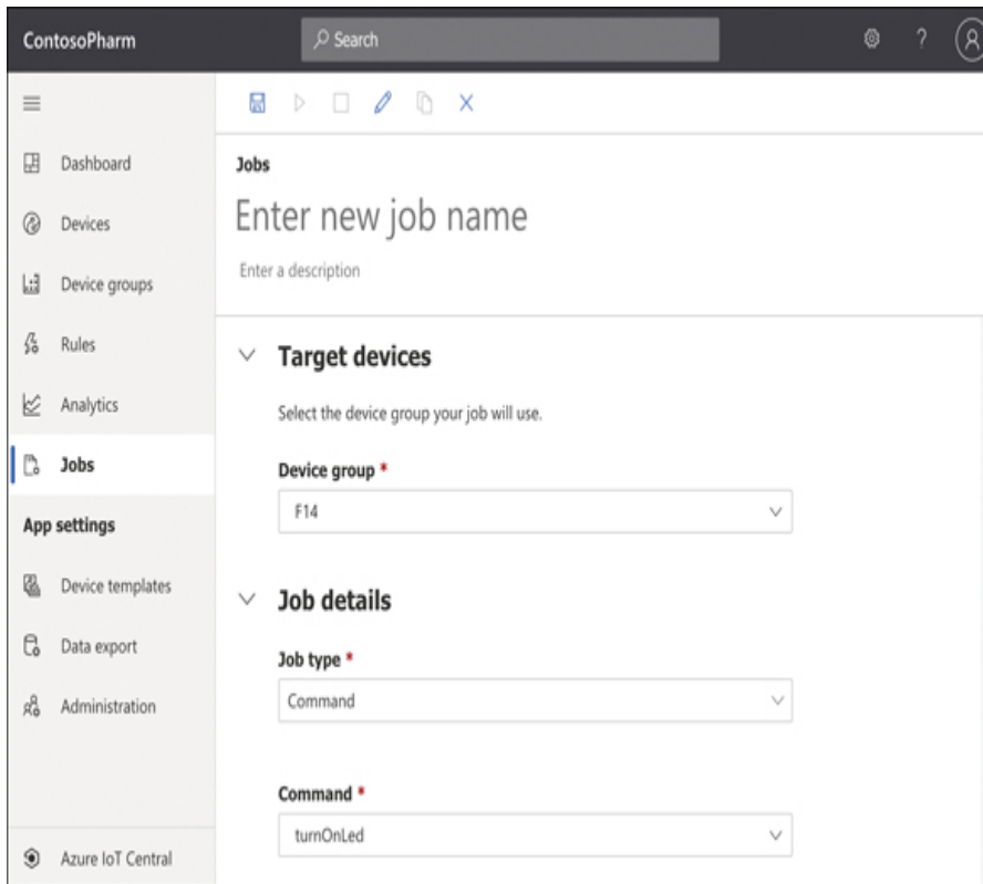
FIGURE 3-14 Creating a job
