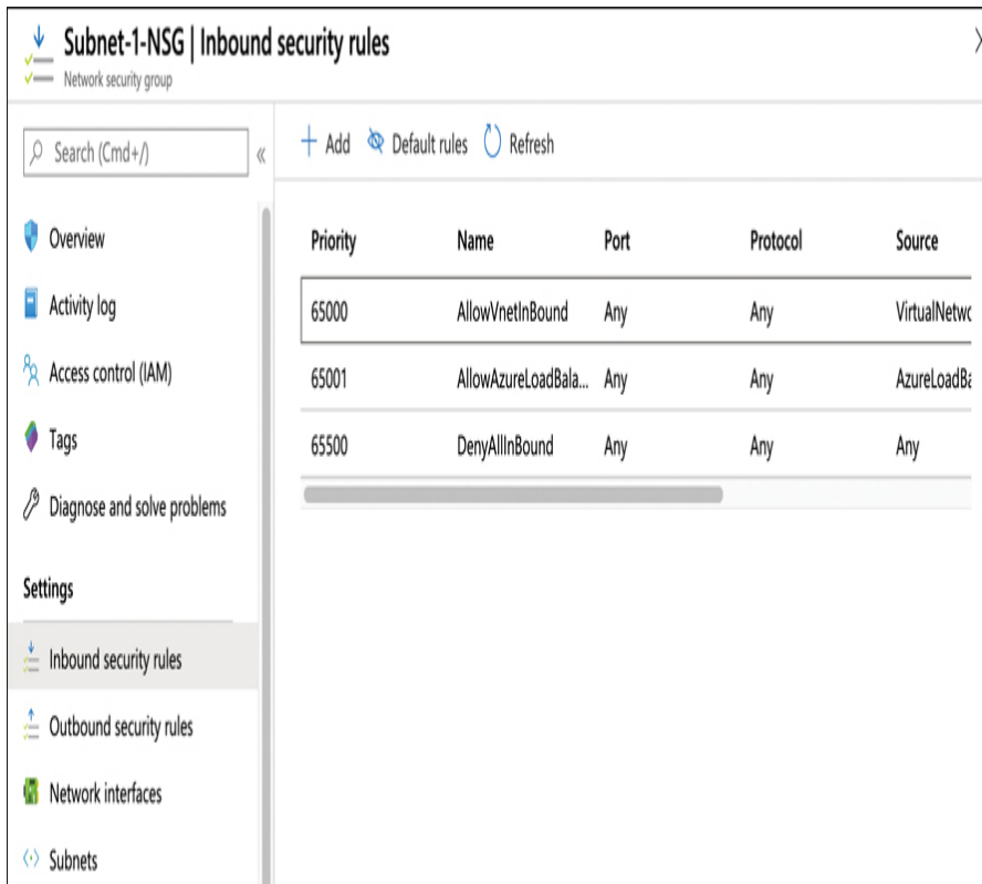
FIGURE 4-23 Inbound Security Rules for an NSG
