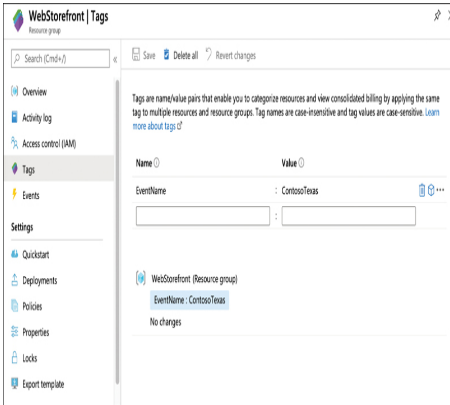
FIGURE 5-26 Tagging a resource group
