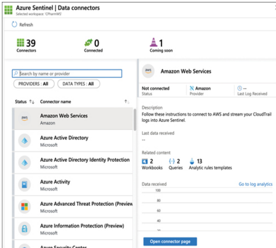
FIGURE 4-14 Adding a connector in Sentinel
