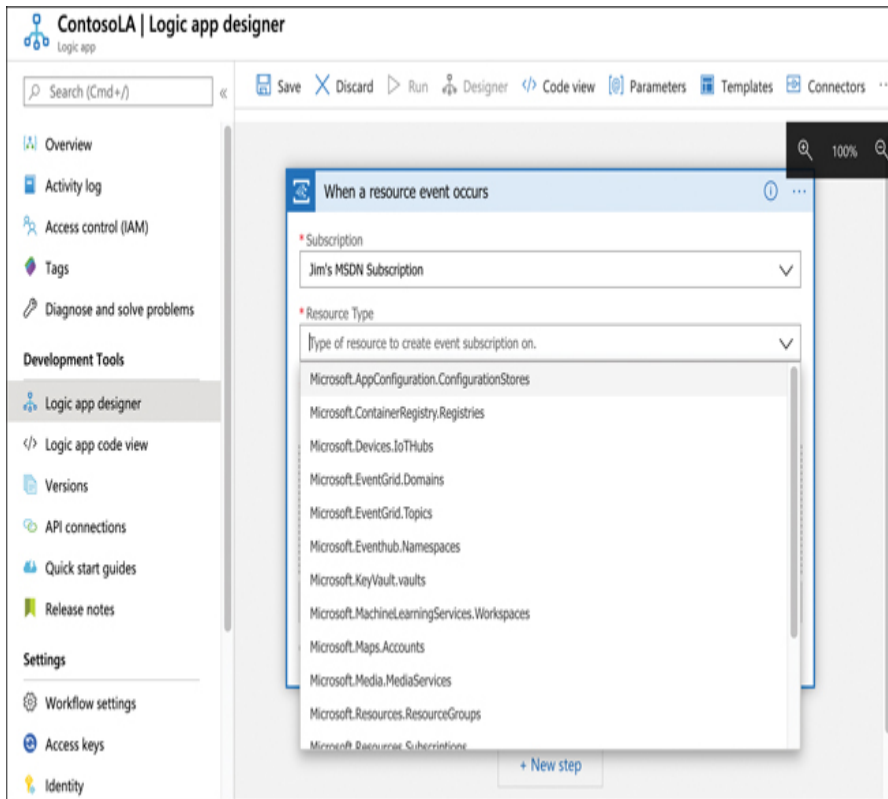
FIGURE 3-46 Resources available in Event Grid
