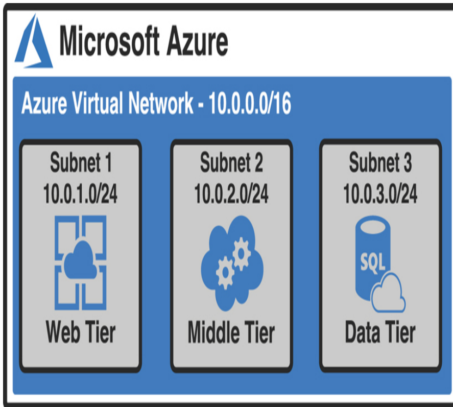
FIGURE 2-27 A multi-tier application in an Azure Virtual Network
