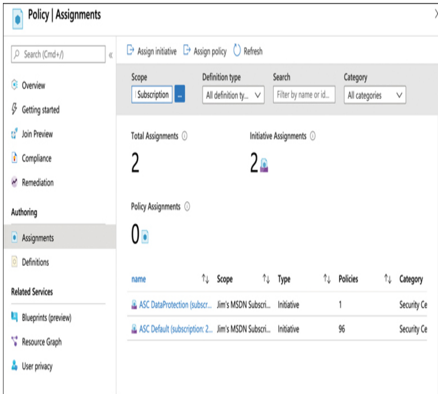
FIGURE 5-18 Assigning a policy
