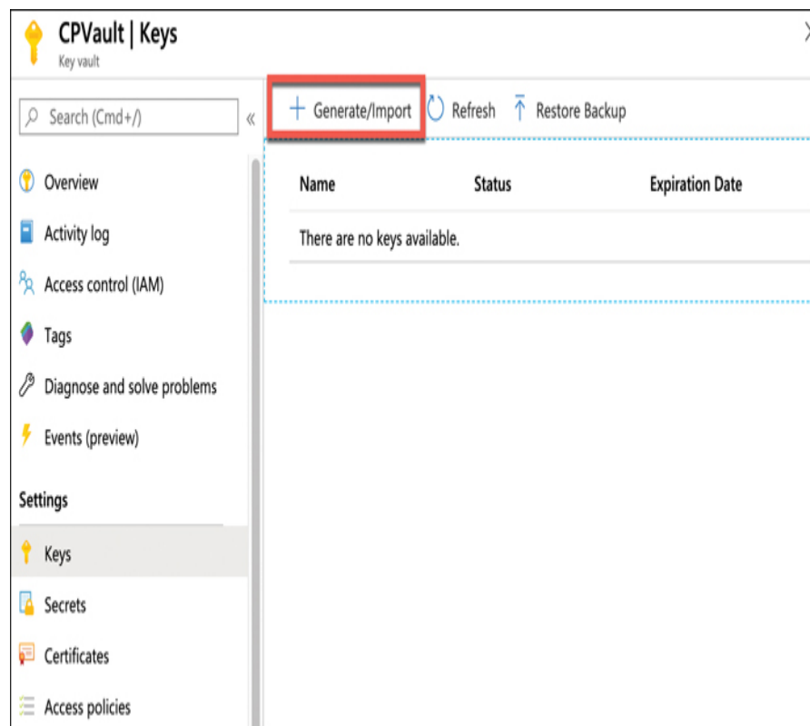
FIGURE 4-8 Adding a key to Key Vault
