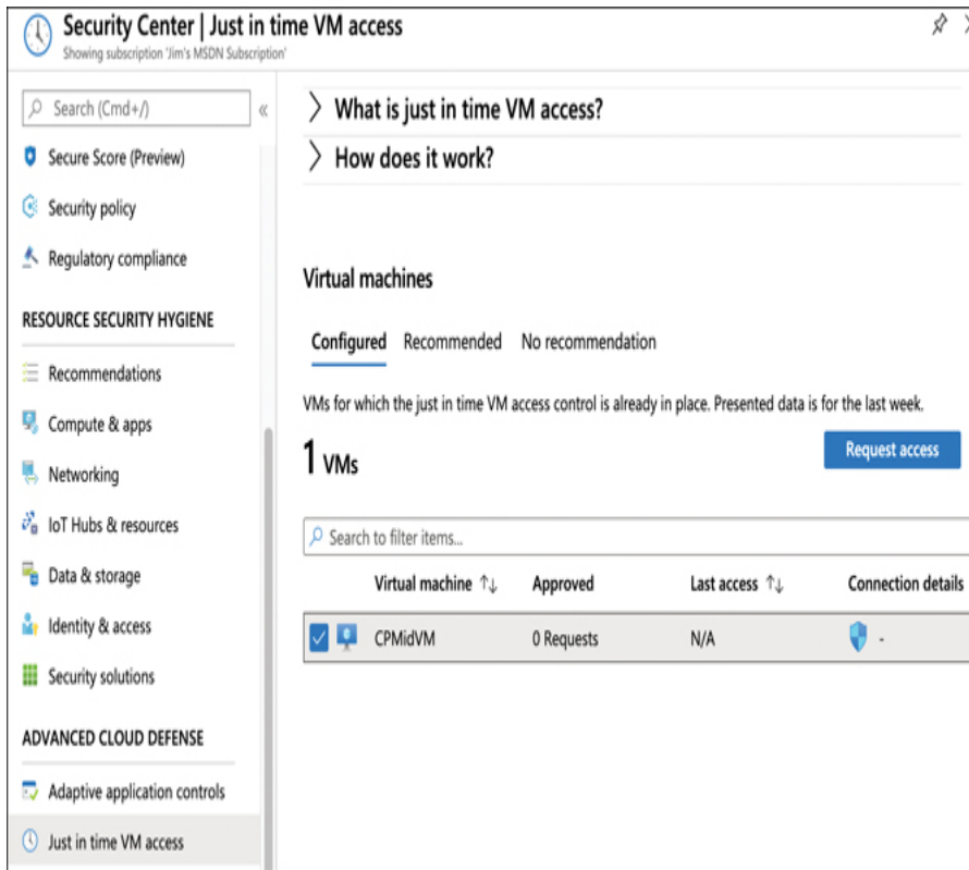
FIGURE 4-5 Requesting JIT access
