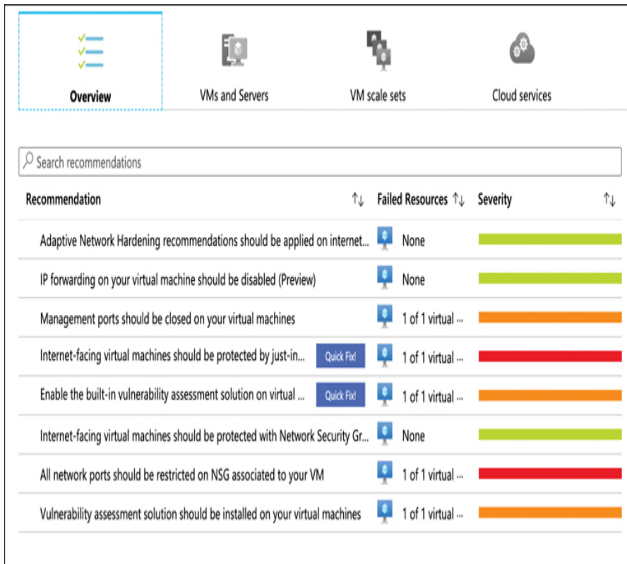
FIGURE 4-2 Overview of all Azure Compute recommendations in Security Center
