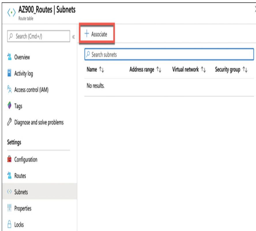
FIGURE 4-30 Associating a route table with a subnet
