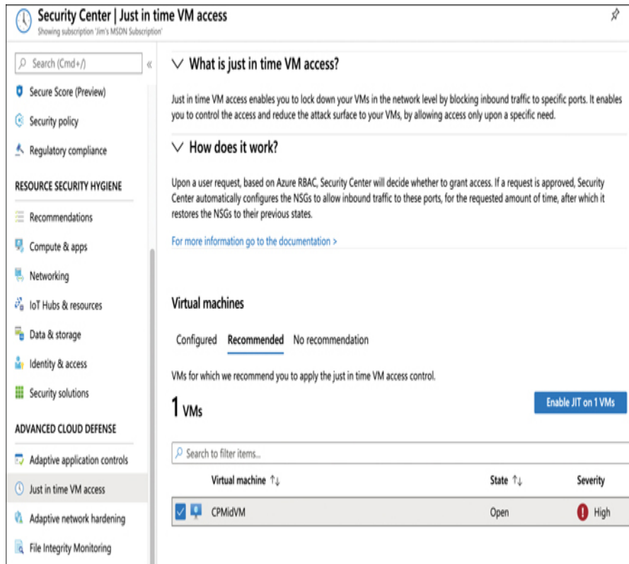
FIGURE 4-3 Enabling JIT access on a VM
