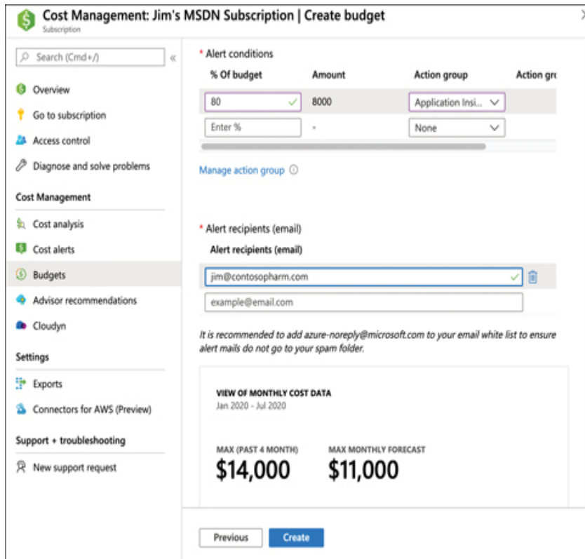
FIGURE 6-12 Configuring alerts for a budget
