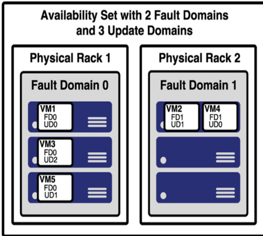
FIGURE 2-18 A better representation of an availability set
