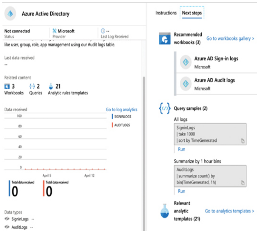
FIGURE 4-16 Next Steps to configure the Azure Active Directory connector in Sentinel
