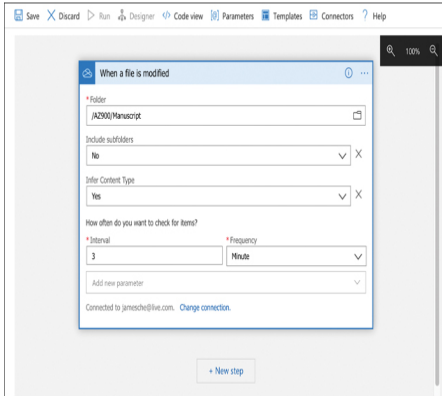
FIGURE 3-42 Using the OneDrive connector
