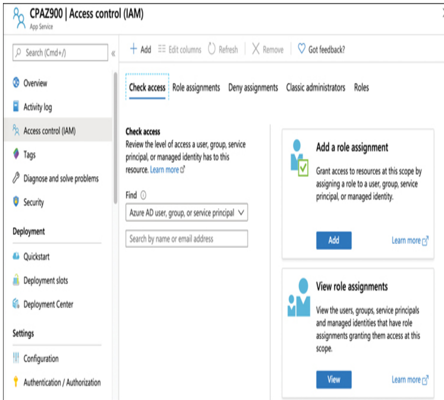
FIGURE 5-11 Configuring RBAC for a web app
