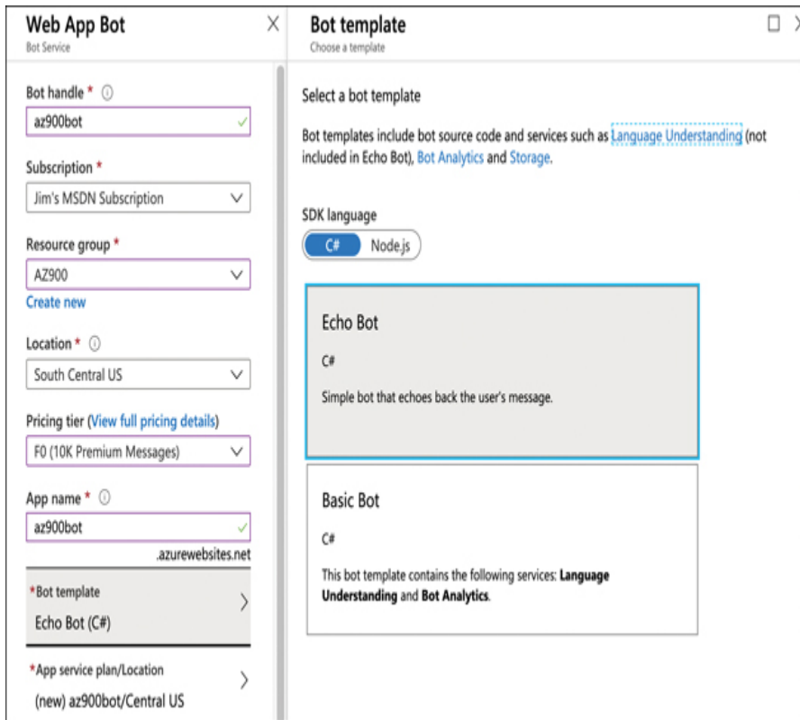
FIGURE 3-27 Creating a bot in Azure Bot Service
