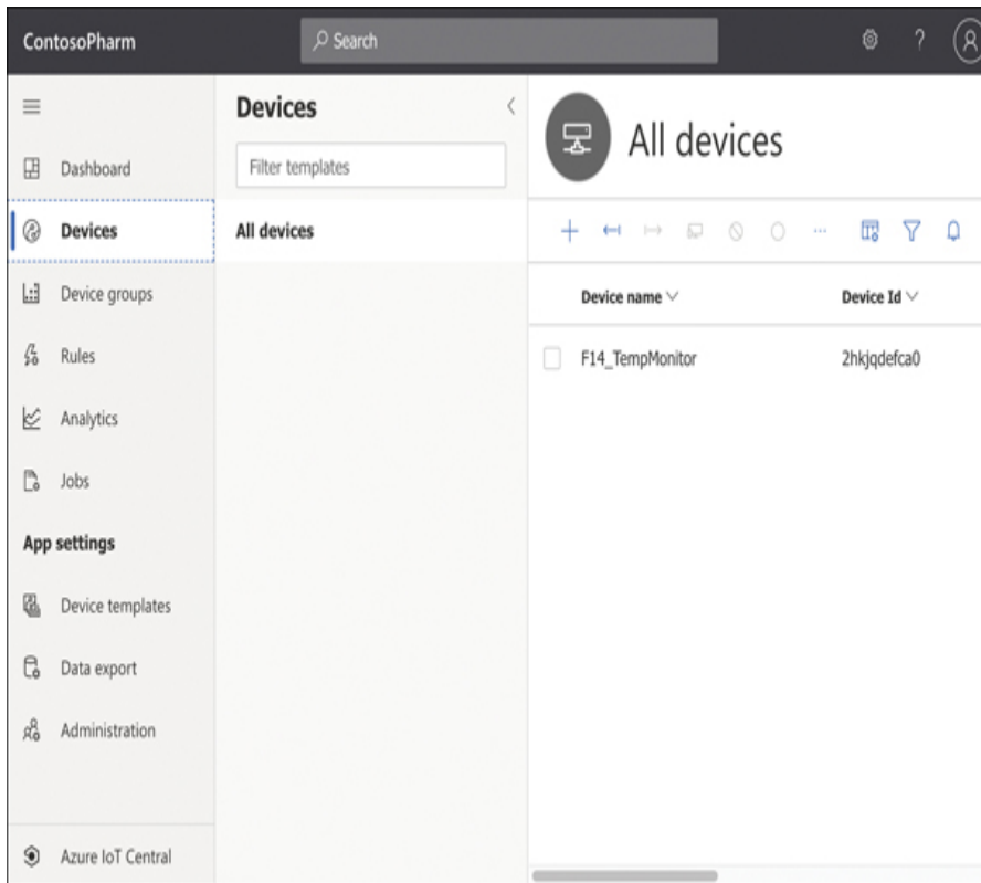
FIGURE 3-7 An IoT device in IoT Central
