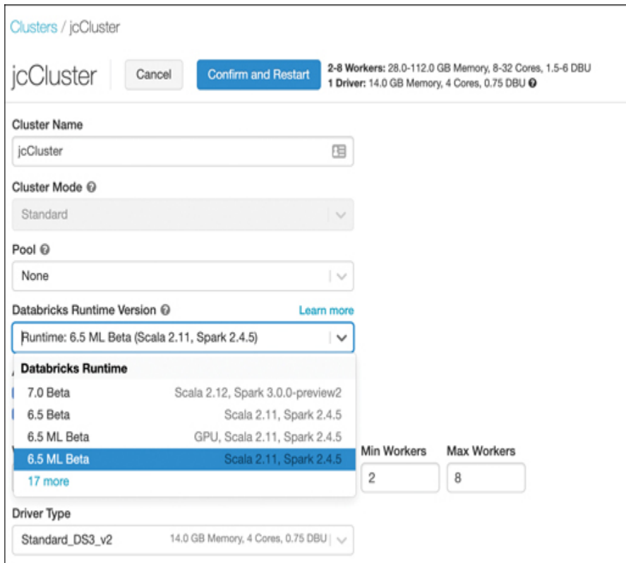
FIGURE 3-24 Databricks Runtime ML in cluster configuration
