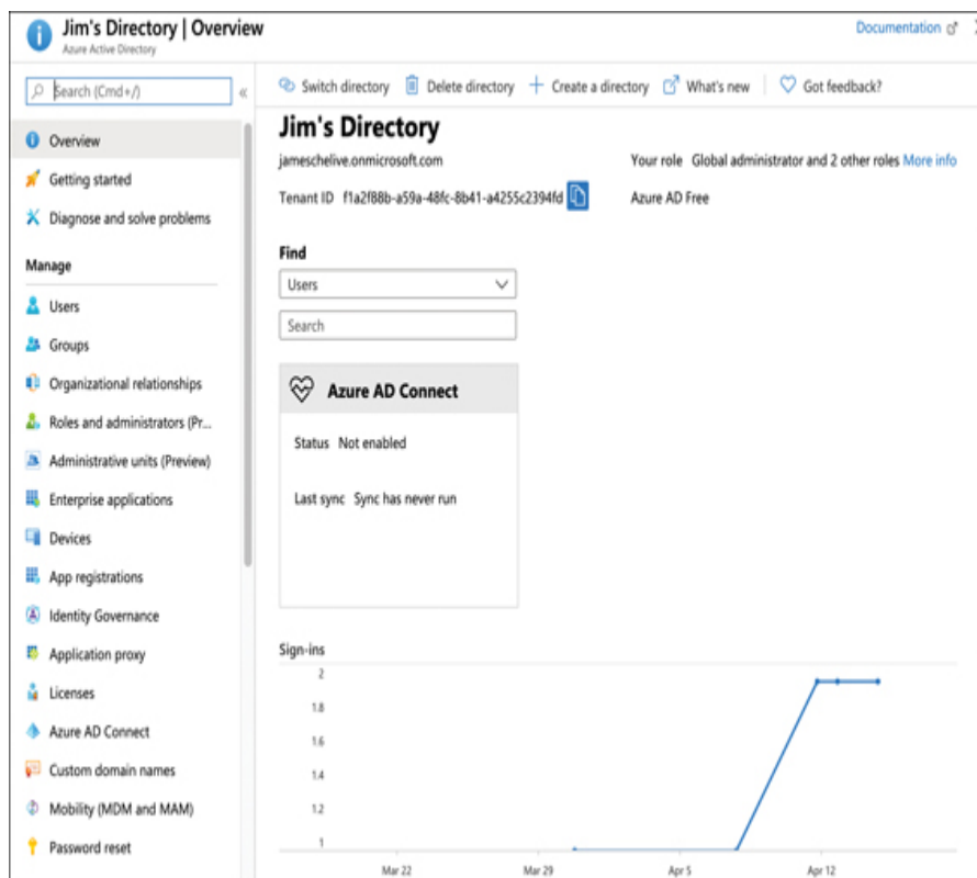
FIGURE 5-1 Azure AD in the Azure portal
