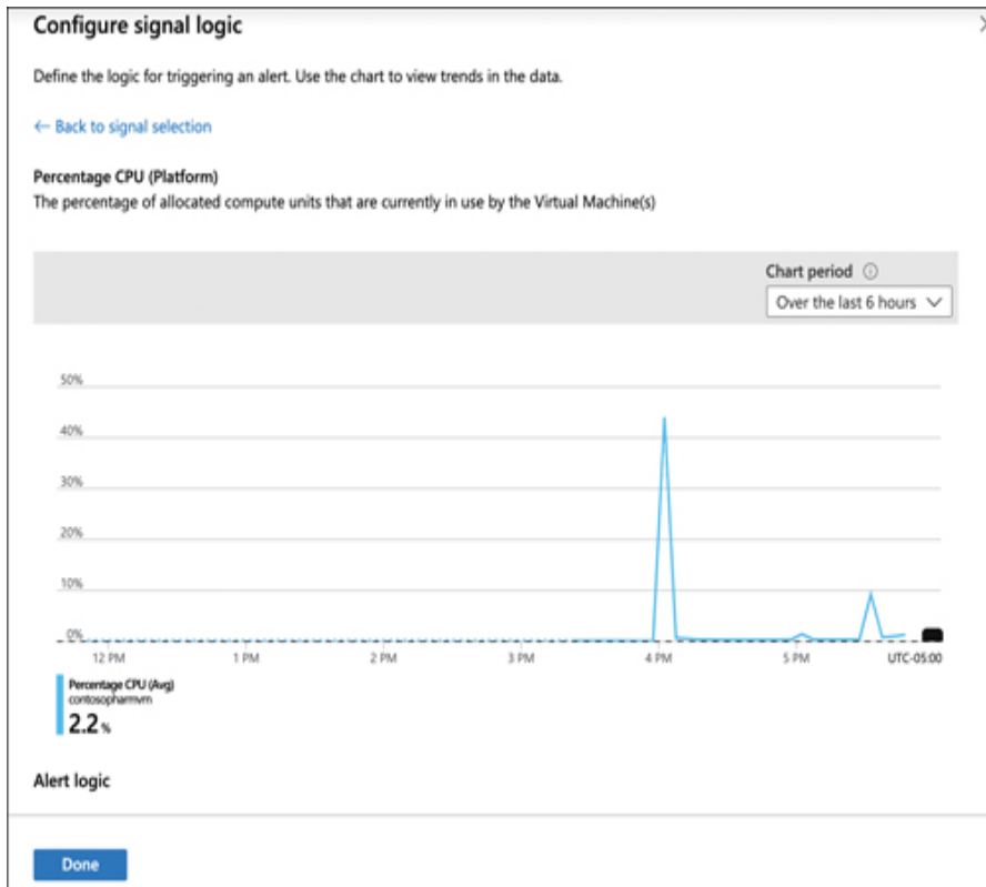
FIGURE 3-96 Alert rule logic
