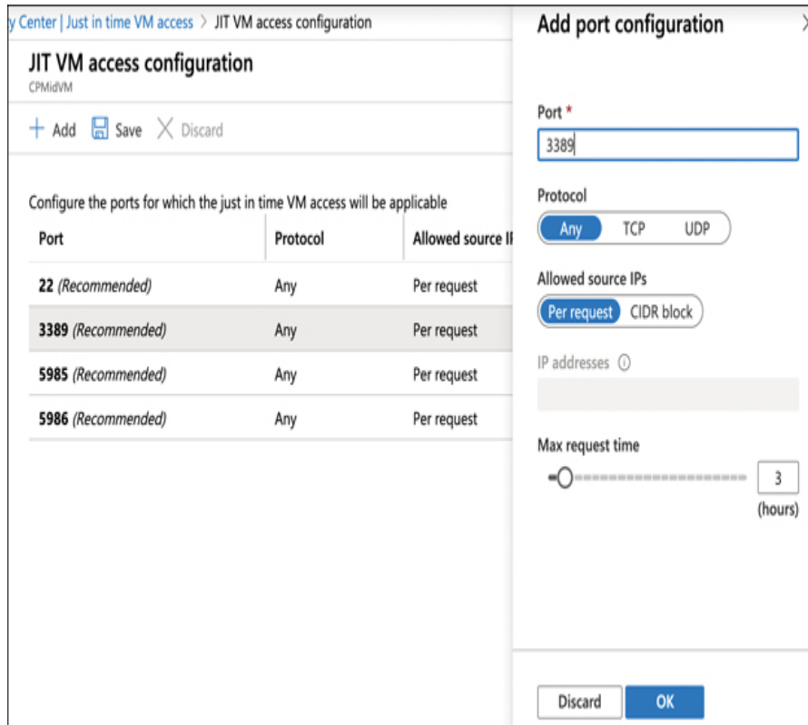
FIGURE 4-4 JIT access configuration
