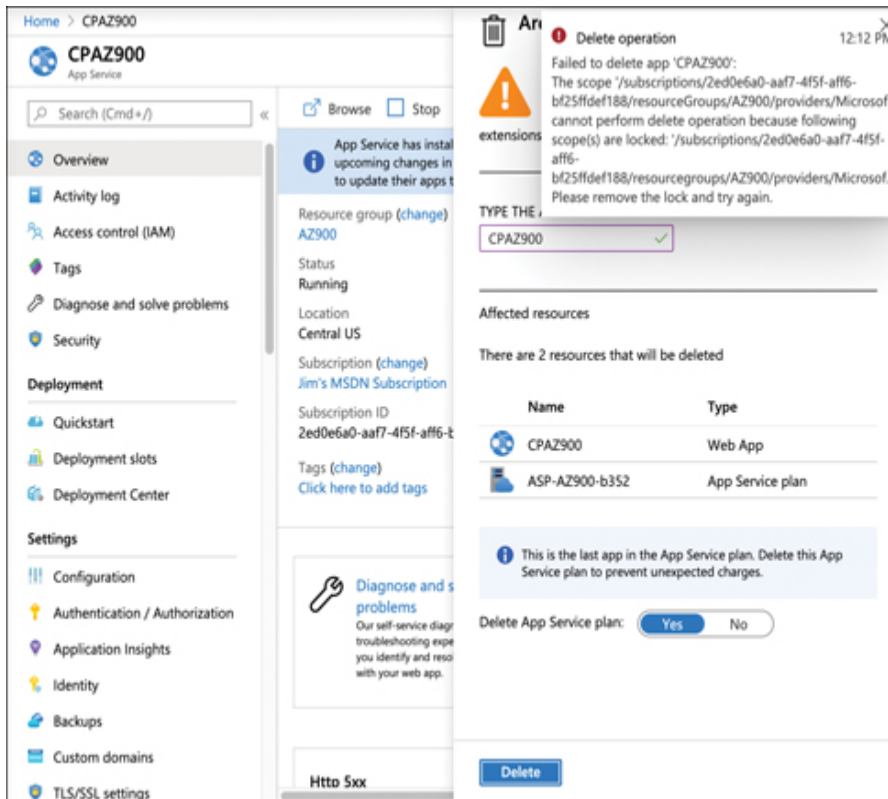
FIGURE 5-24 Denied by a lock
