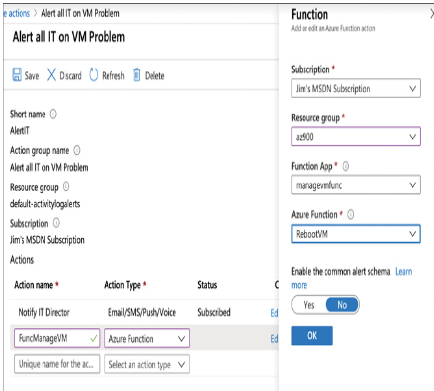
FIGURE 3-99 Adding another action
