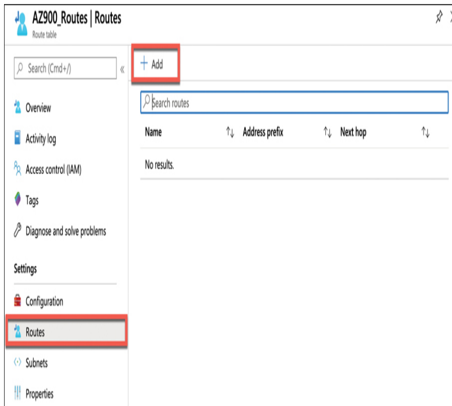
FIGURE 4-32 Adding a new user-defined route to the route table
