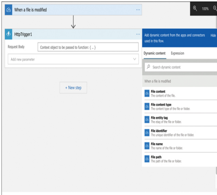
FIGURE 3-44 Configuring a Function App action
