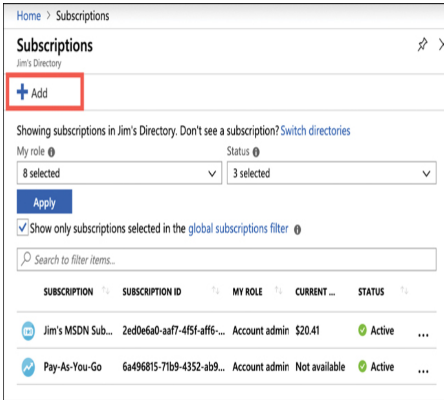
FIGURE 2-8 Creating a new subscription
