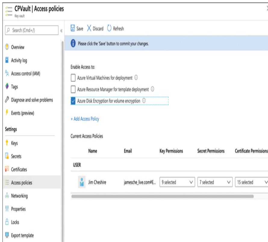
FIGURE 4-11 Setting access policies to allow access to Azure Disk Encryption
