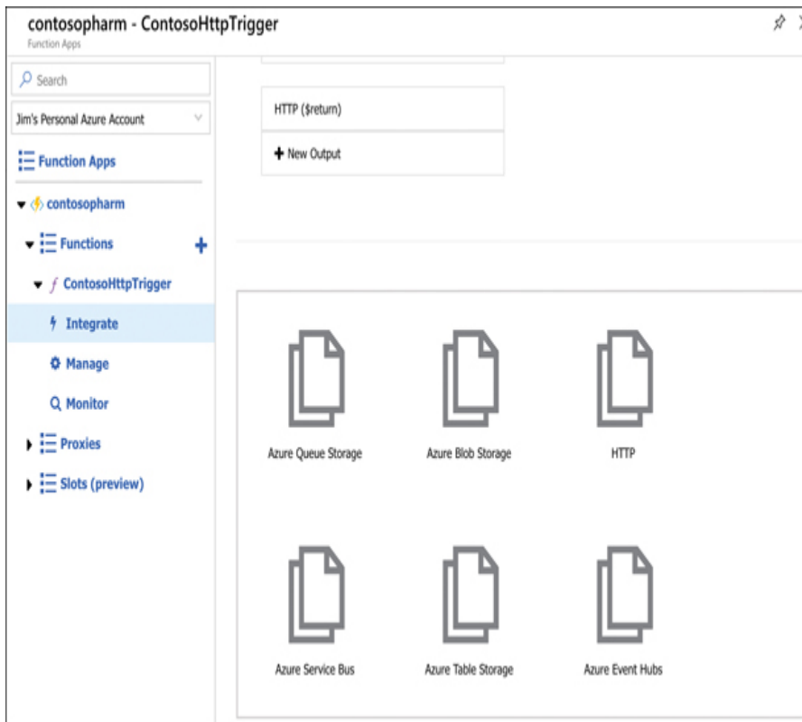
FIGURE 3-38 Output bindings in Azure Functions
