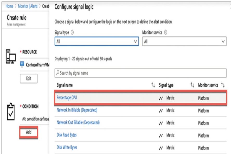
FIGURE 3-95 Configuring a condition
