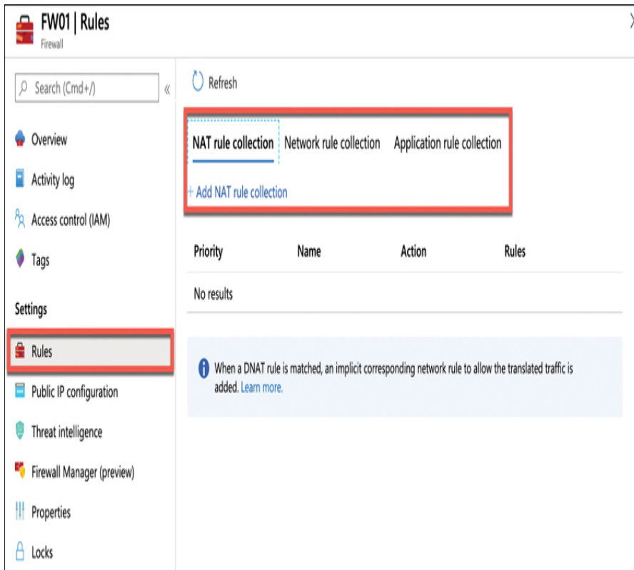
FIGURE 4-34 Azure Firewall rule collections in the Azure portal
