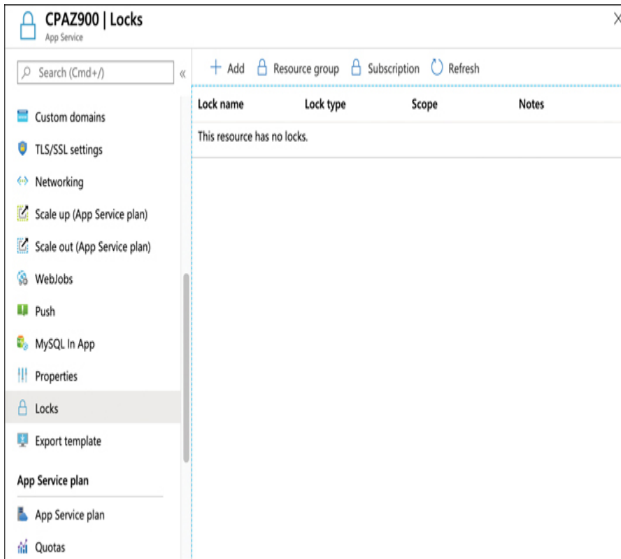
FIGURE 5-22 Locking a resource
