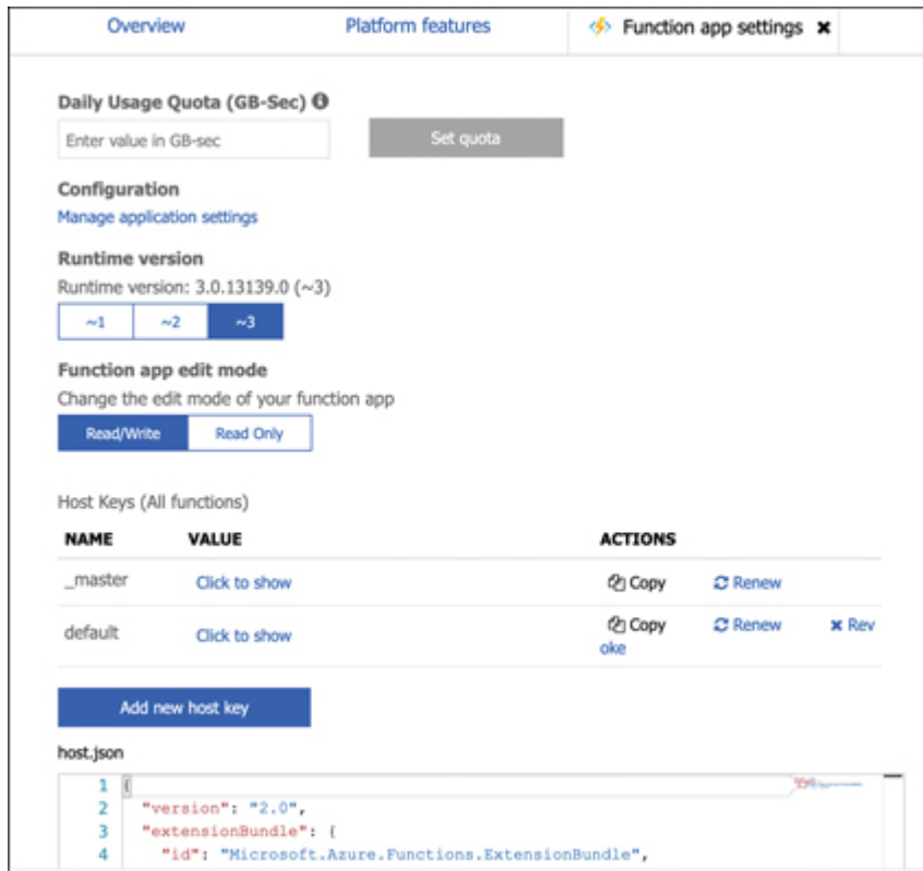
FIGURE 3-33 Function App settings
