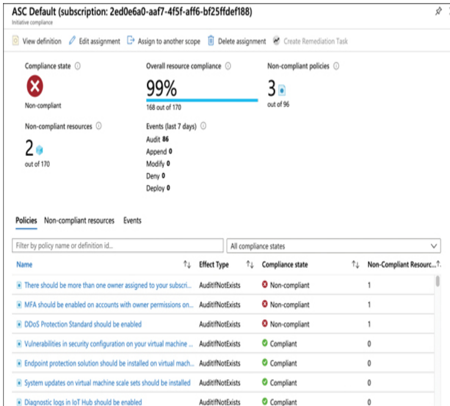
FIGURE 5-17 Details on compliance
