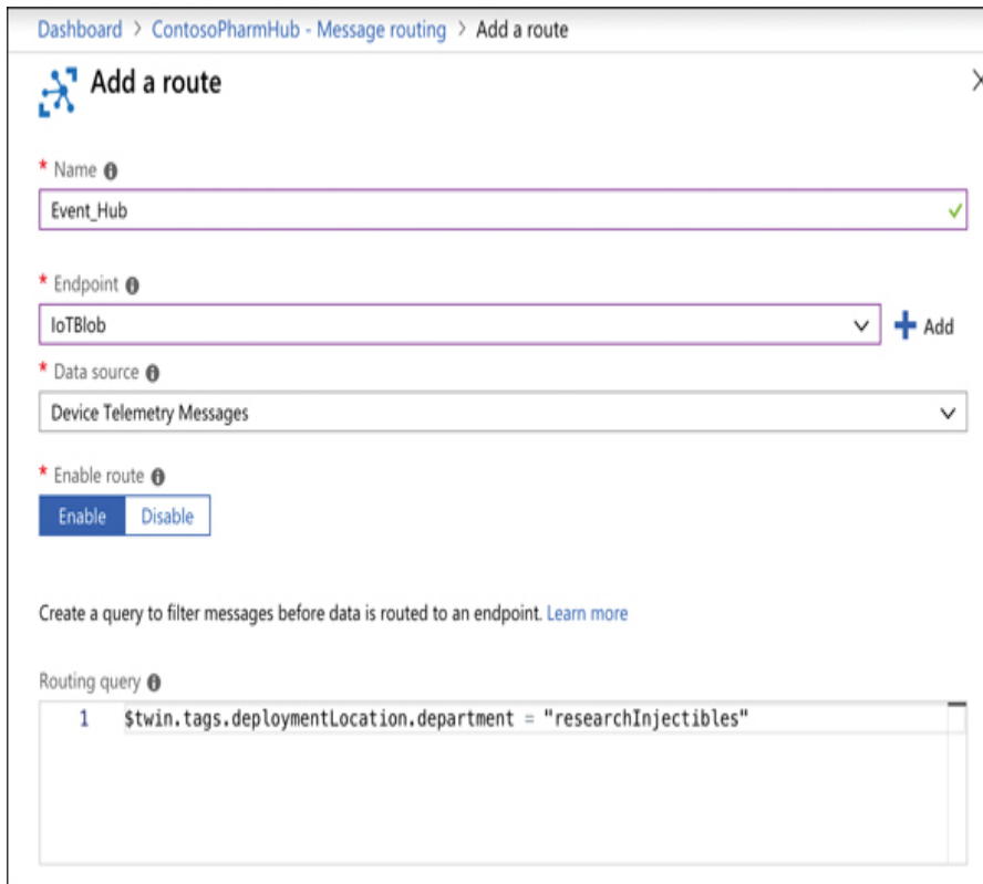
FIGURE 3-3 Adding a message route in IoT Hub
