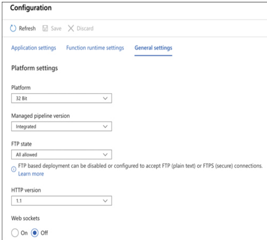
FIGURE 3-34 Some of the Function App settings
