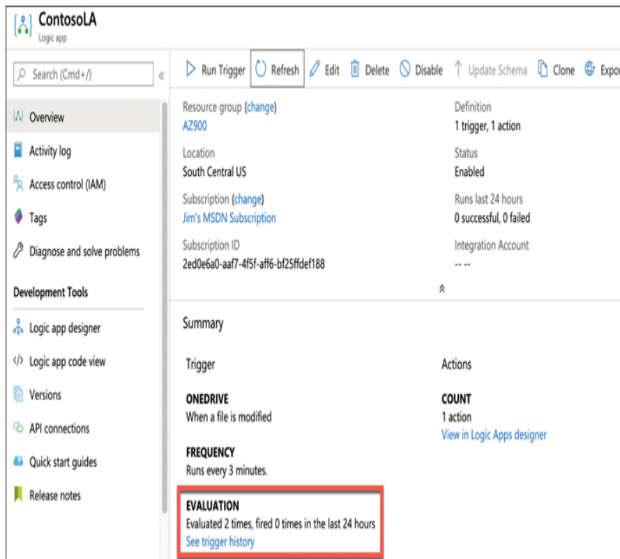
FIGURE 3-45 The Azure portal displaying when the Logic App flow ran
