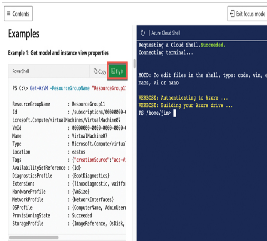
FIGURE 3-79 Cloud Shell’s integration with Microsoft documentation
