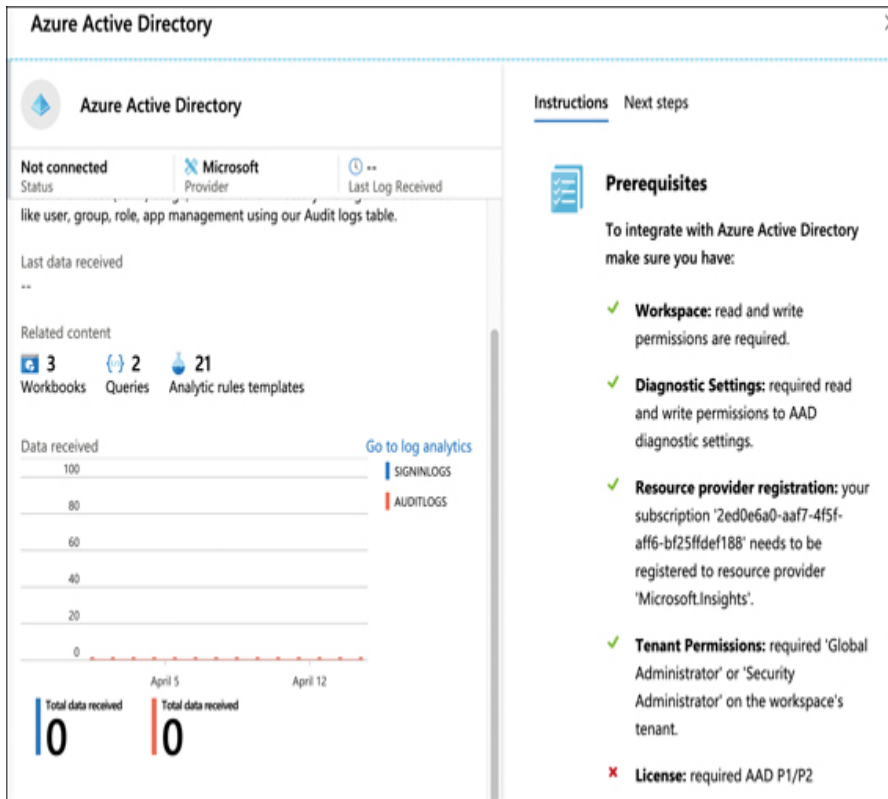
FIGURE 4-15 The Azure Active Directory connector in Sentinel
