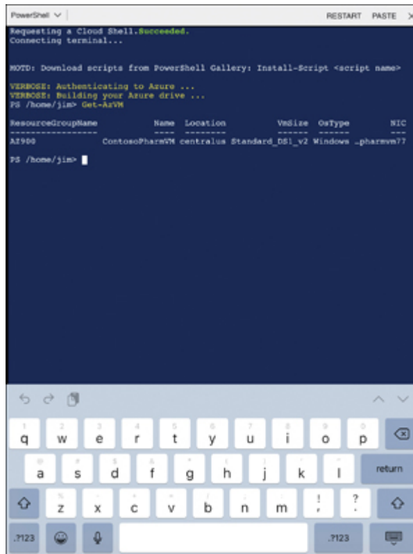
FIGURE 3-82 Cloud Shell running in Azure mobile app
